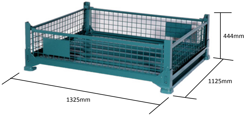
Assembled state
