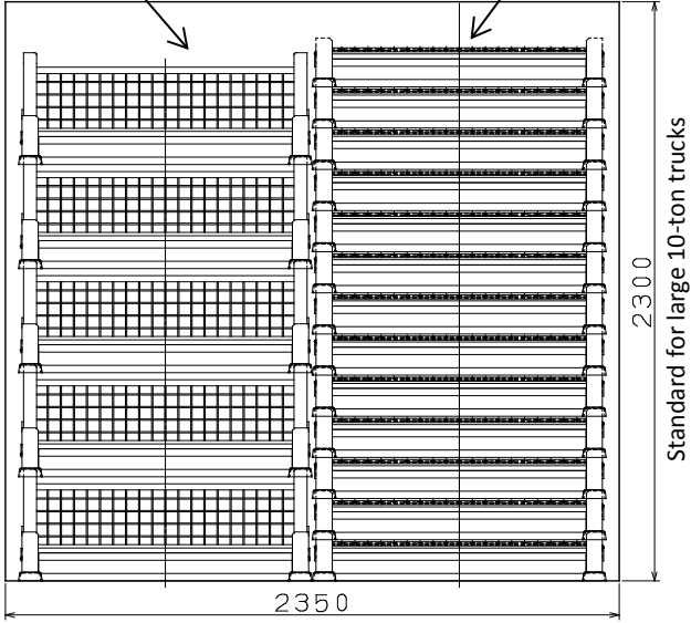
Loaded state on a 10-ton large truck
